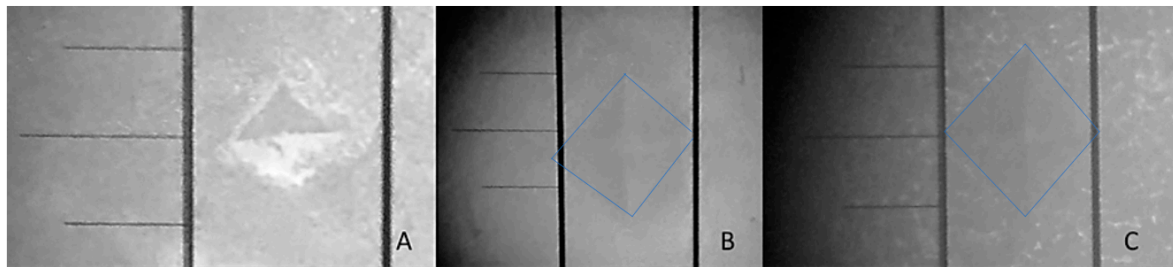
Figure 2. (A) Indentation from Group B; (B) Indentation from Group D where the mark is bigger than the previous image, (C) Indentation from Group F, showing a softer surface for a greater indentation.
